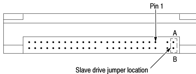
Figure 3-1: Slave drive jumper location
