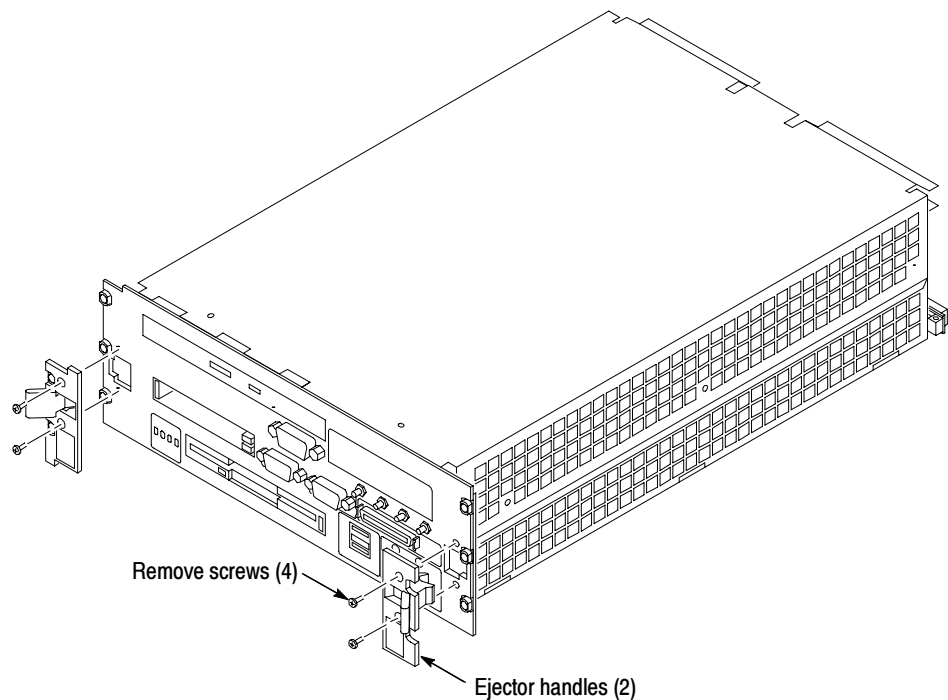
Figure 7- 11: Removing the ejector handles
