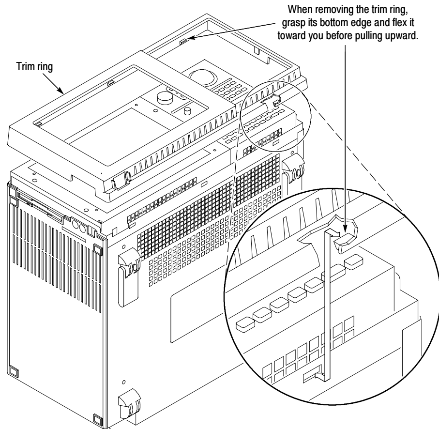
Figure 7-1: Trim ring removal
